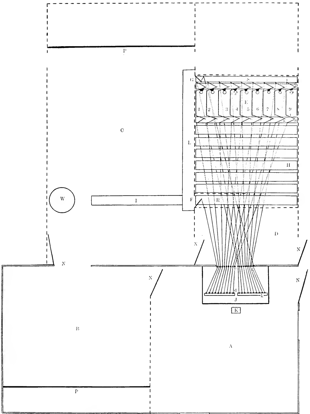
FIGURE 2. Ground plan of crow house, fly, and apparatus. Scale, \frac{1}{4} . A, observation room; B, bird room; C, main portion of fly; D, passageway for experimenter; E, multiple choice box; F, entrance door between main fly, C, and alley to reaction chamber, H; G, exit door between alley S and main fly; H, reaction chamber, the floor boards of which are separated somewhat; I, L, approaches to the doors F and G; J, observer's table and key-board; K, observer's stool; N, doors for experimenter's use; P, perches; R, alley leading to middle of reaction chamber H; S, alley leading from exits to main fly; W, water tub for crows.
